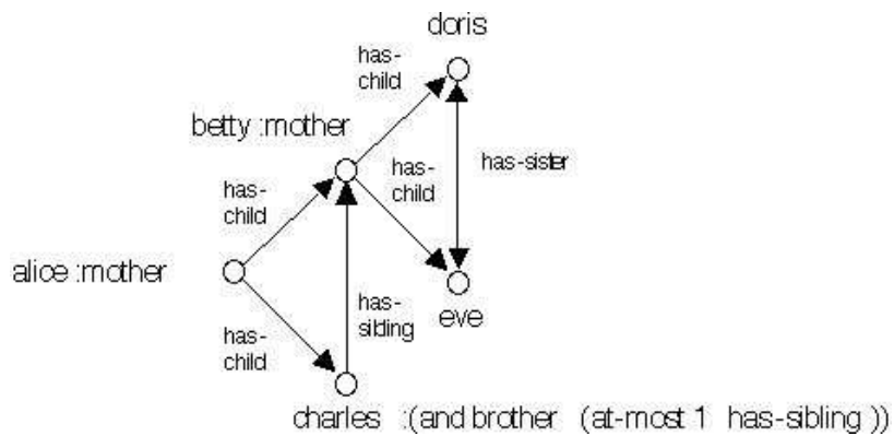
Figure 3: Depiction of the ABox smith-family. (with explicitly given information being shown)
