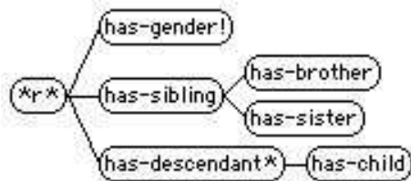
Figure 1: Role hierarchy for the family TBox. * r * denotes the internally defined universal role. ! denotes features * denotes transitive roles
