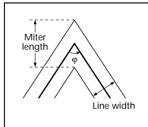
Figure 8.6 Miter length
