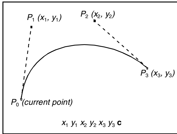
Figure 8.7 Bézier curve
